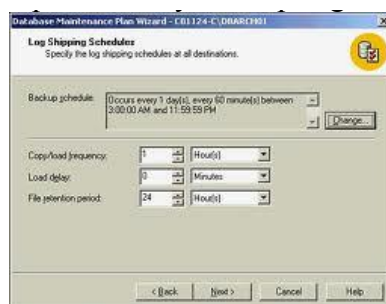
Rys.18. Log shipping
